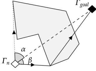
Figure 3: The heuristic for a point with an obstructed line of sight due to a non-convex wind hazard polygon involves calculating the distance to the nearest extreme point on the obstructing polygon with the smallest angle, followed by the distance to the goal. This path is denoted by \beta , while the path \alpha is not used since the distance \theta_\alpha > \theta_\beta .
